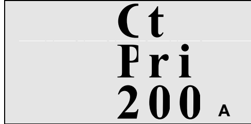
Figure 4.1 Setting The CT Primary Constant
