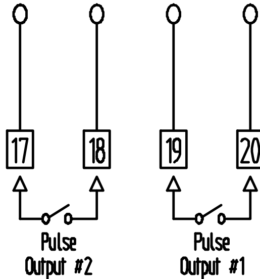
Figure 2.2 Pulse Output Connection
