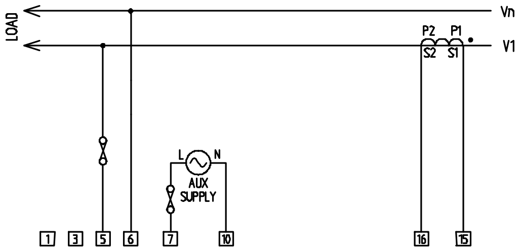
Figure 3.5 Single Phase
