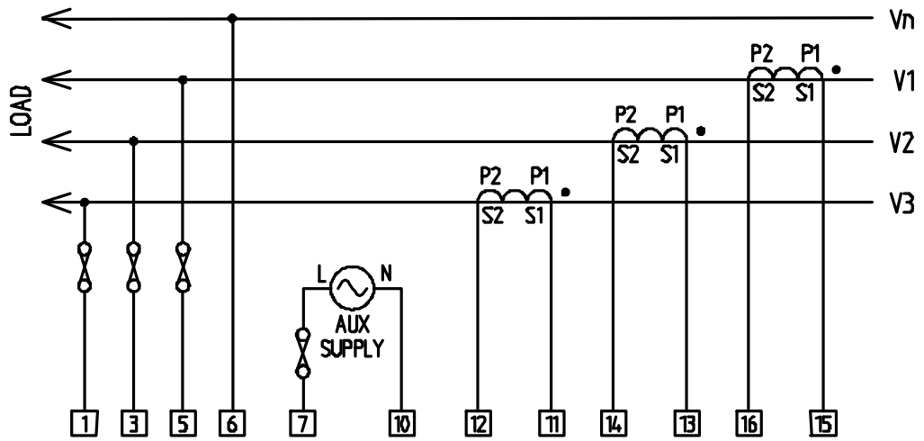
Figure 3.4 3-Phase 4-Wire
