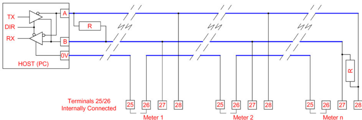
Figure 3-1 Basic RS485 To Internal Modbus Option
